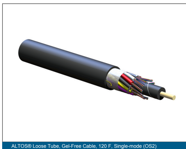
ALTOS® Loose Tube, Gel-Free Cable, 120 F, Single-mode (OS2)
